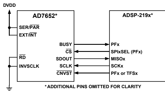
Figure 37. Interfacing the AD7652 to an SPI Interface
