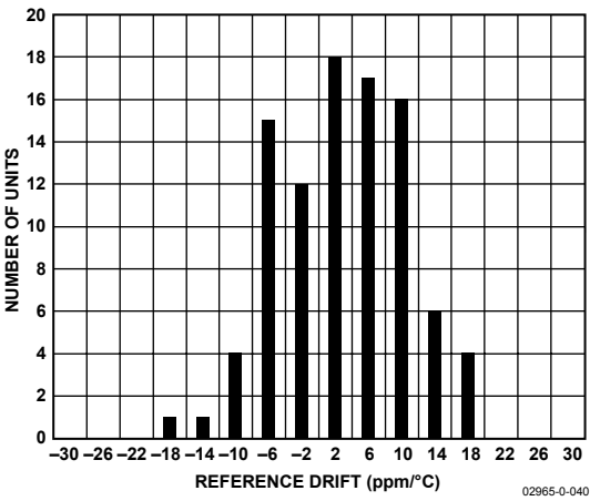
Figure 18. Reference Voltage Temperature Coefficient Distribution (100 Units)
