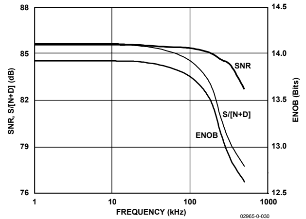
Figure 10. SNR, S/[\text{N}+\text{D}] , and ENOB vs. Frequency
