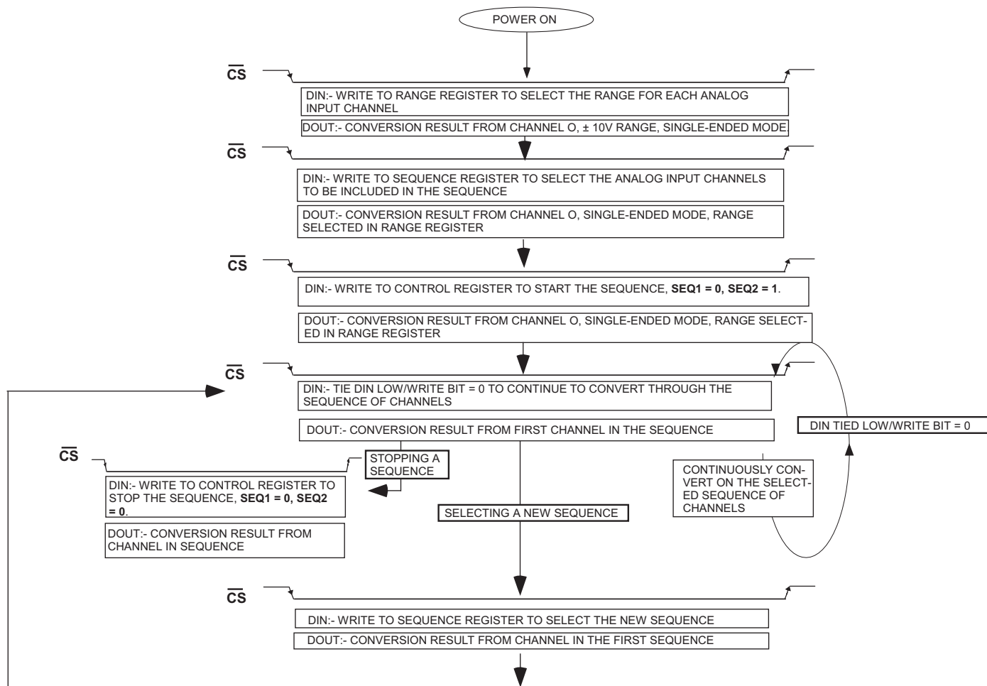
Figure 13. Programmable sequence Flow Chart
