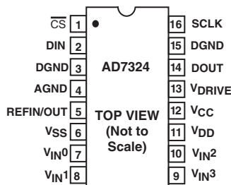
Figure 3. AD7324 Pin Configuration TSSOP
