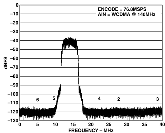
TPC 27. WCDMA Tone 140 MHz: Encode = 76.8 MSPS
