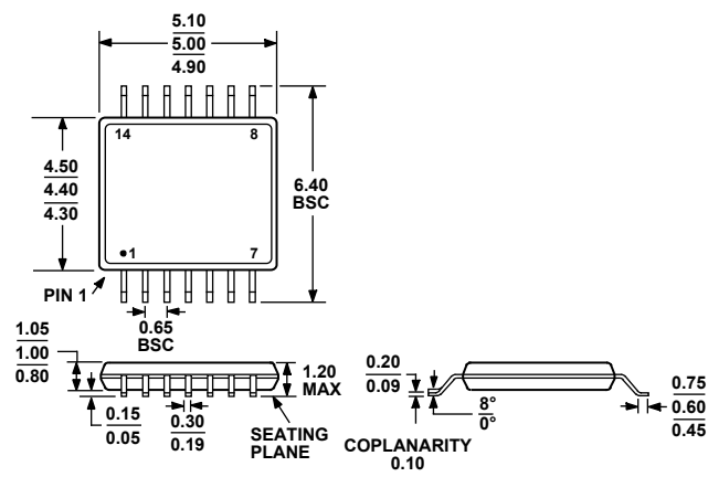
COMPLIANT TO JEDEC STANDARDS MO-153-AB-1 Figure 58. 14-Lead Thin Shrink Small Outline Package [TSSOP] (RU-14) Dimensions shown in millimeters
