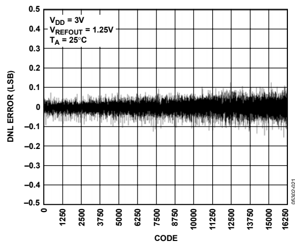
Figure 21. DNL AD5648-1
