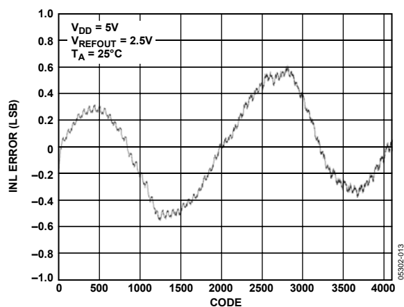
Figure 13. INL AD5628-2
