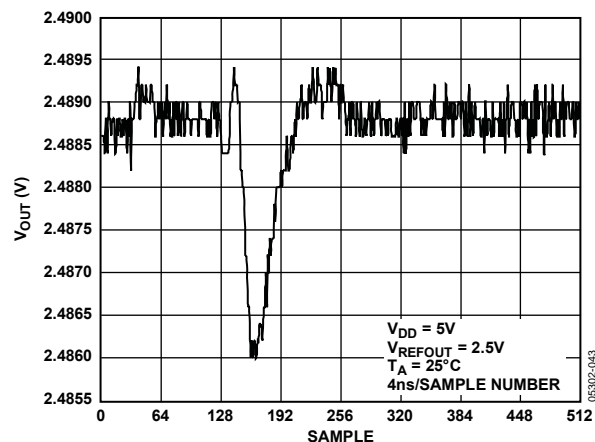
Figure 42. DAC-to-DAC Crosstalk
