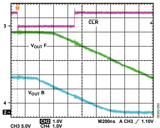
Figure 49. Hardware \overline{CLR}
