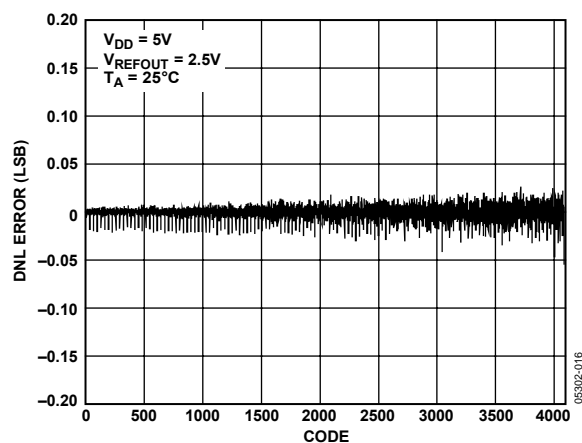
Figure 16. DNL AD5628-2
