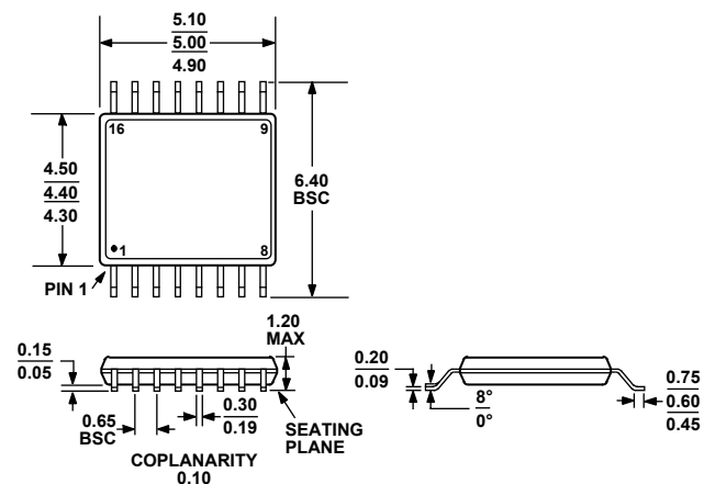
COMPLIANT TO JEDEC STANDARDS MO-153-AB Figure 59. 16-Lead Thin Shrink Small Outline Package [TSSOP] (RU-16) Dimensions shown in millimeters
