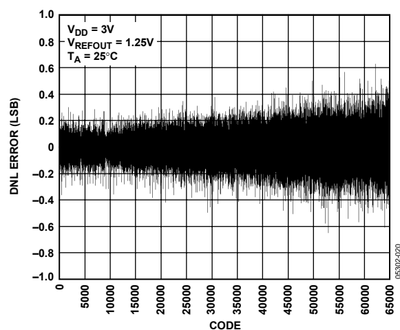
Figure 20. DNL AD5668-1
