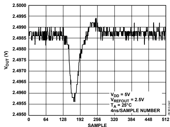
Figure 41. Analog Crosstalk
