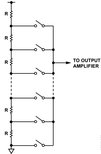
Figure 52. Resistor String
