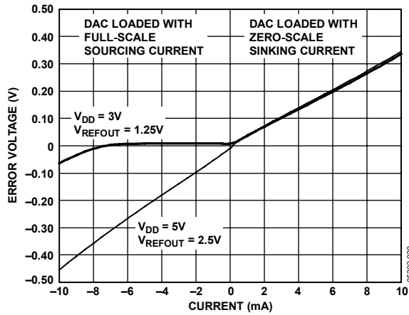
Figure 29. Headroom at Rails vs. Source and Sink
