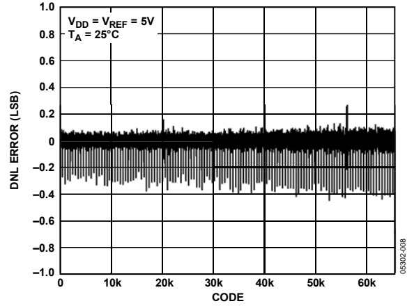
Figure 8. DNL AD5668—External Reference
