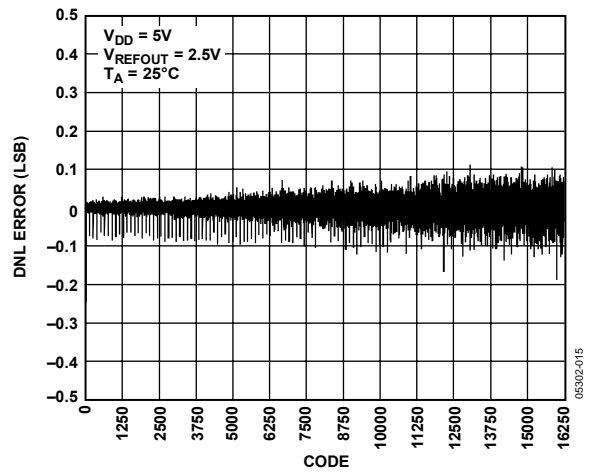
Figure 15. DNL AD5648-2
