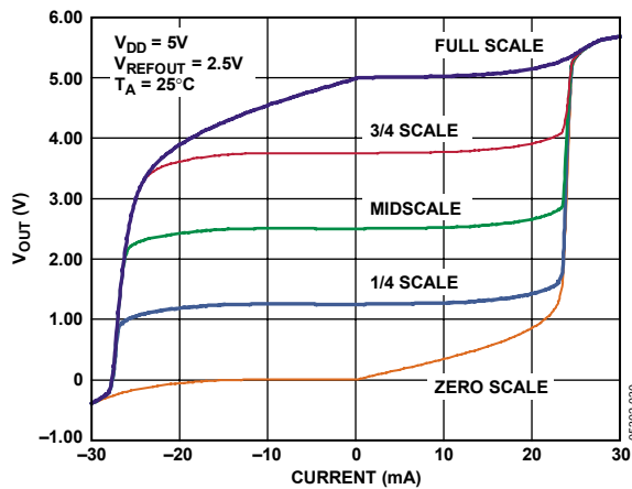
Figure 30. AD5668-2/AD5668-3 Source and Sink Capability
