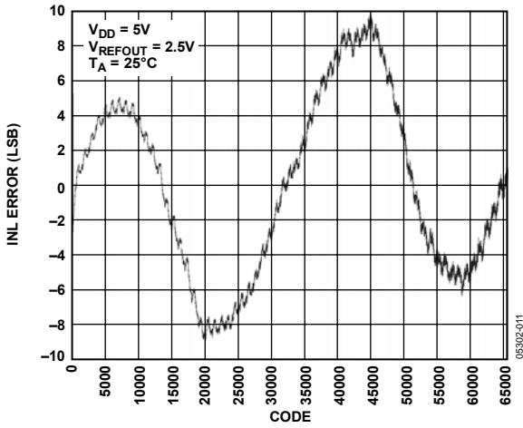
Figure 11. INL AD5668-2/AD5668-3
