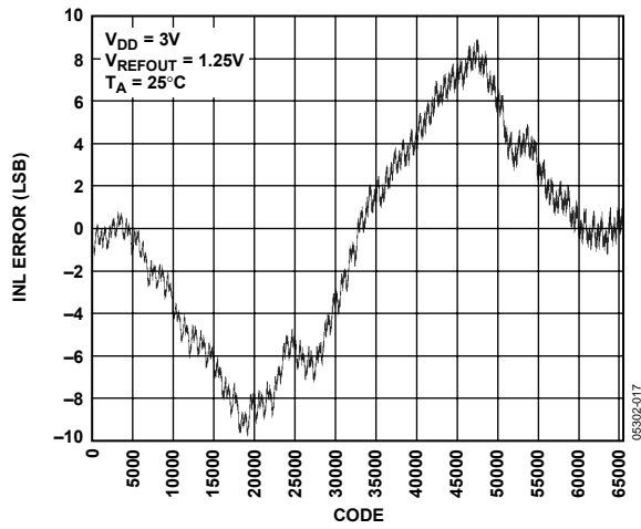
Figure 17. INL AD5668-1
