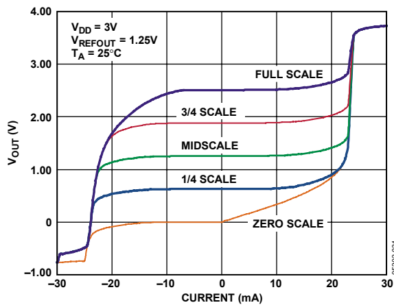
Figure 31. AD5668-1 Source and Sink Capability
