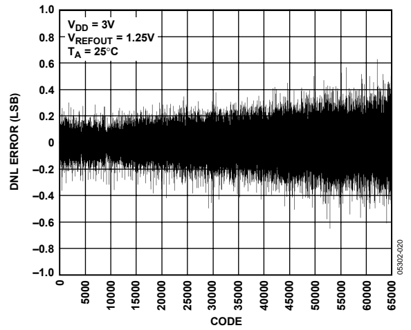
Figure 20. DNL AD5668-1
