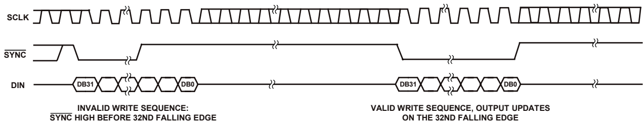
Figure 56. SYNC Interrupt Facility
