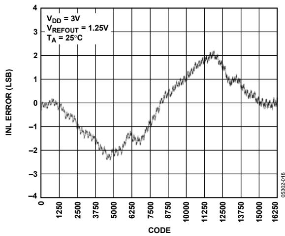
Figure 18. INL AD5648-1
