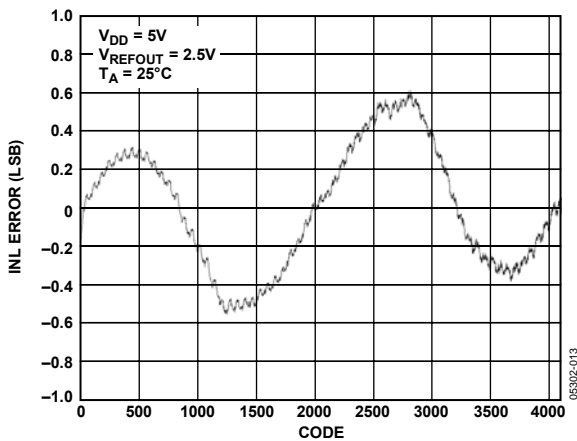
Figure 13. INL AD5628-2
