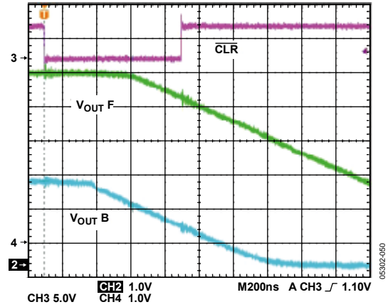
Figure 49. Hardware CLR
