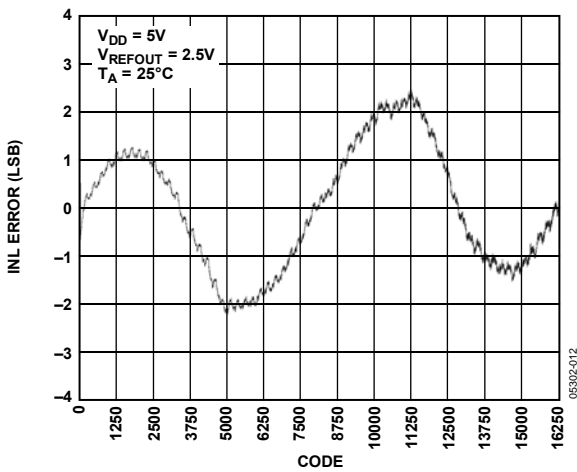
Figure 12. INL AD5648-2
