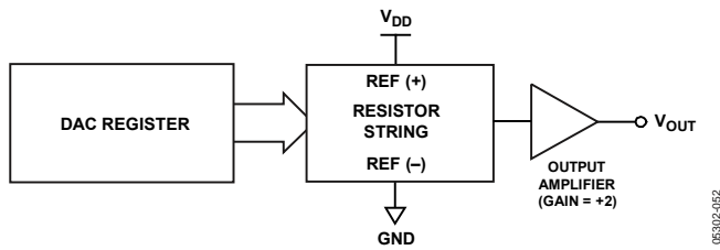
Figure 51. DAC Architecture
