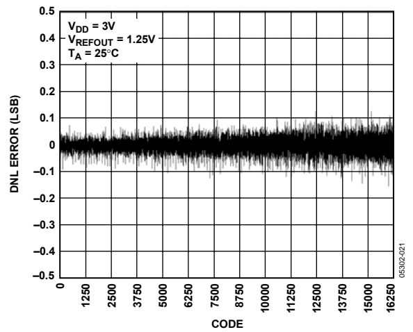
Figure 21. DNL AD5648-1
