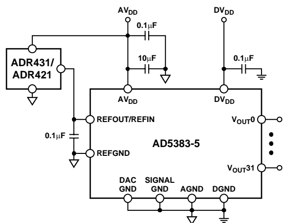
Figure 39. Typical Configuration with External Reference
