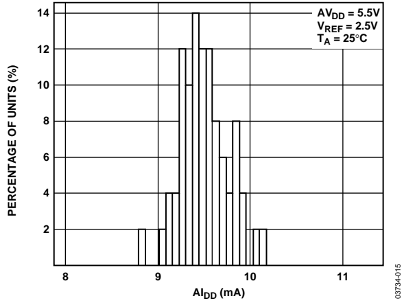
Figure 15. A_{DD} Histogram
