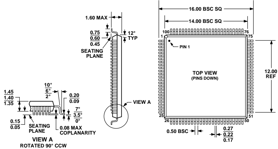
Figure 45. 100-Lead Low Profile Quad Flat Package [LQFP] (ST-100) Dimensions shown in millimeters
