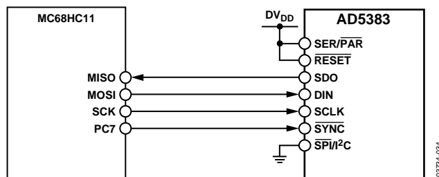
Figure 34. AD5383-to-MC68HC11 Interface
