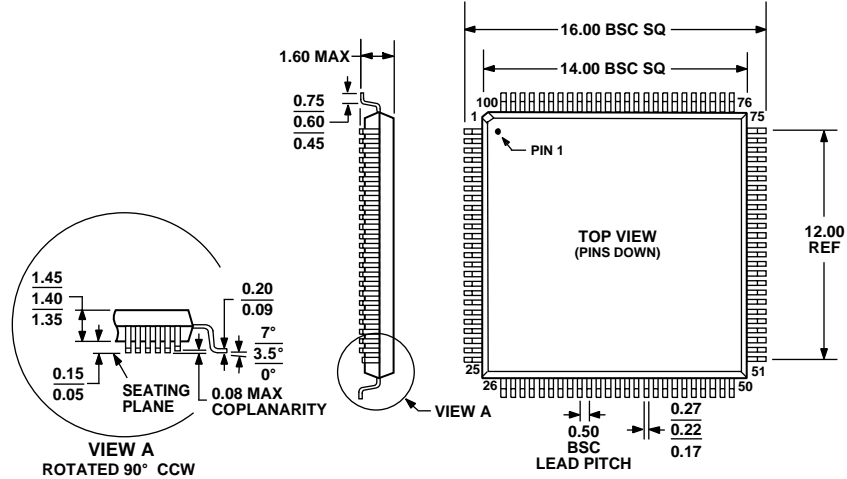
COMPLIANT TO JEDEC STANDARDS MS-026BED Figure 45. 100-Lead Low Profile Quad Flat Package [LQFP] (ST-100) Dimensions shown in millimeters
