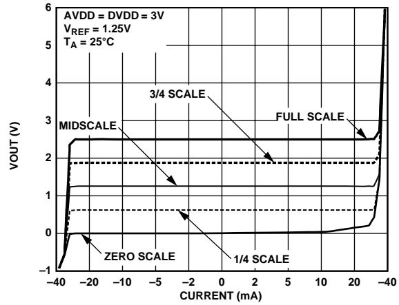
Figure 24. AD5381-3 Output Amplifier Source and Sink Capability
