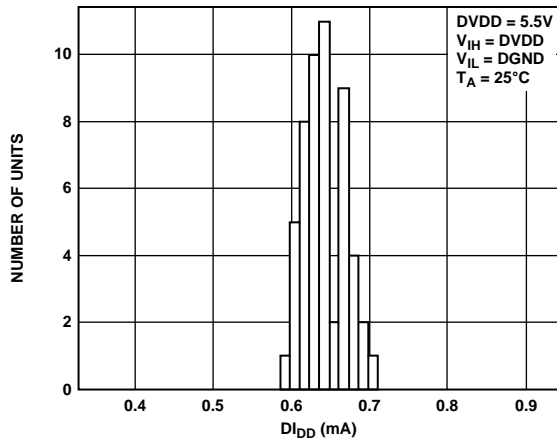
Figure 16. DlDD Histogram
