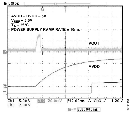
Figure 18. Power-Up Transient
