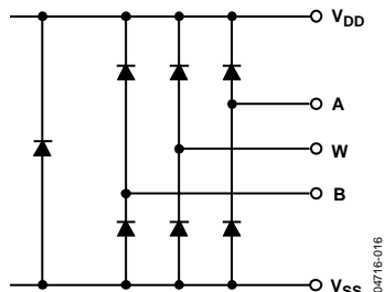
Figure 31. Equivalent ESD Protection Analog Pins
