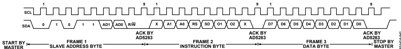
Figure 42. Writing to the RDAC Register
