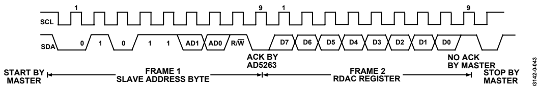
Figure 43. Reading Data from a Previously Selected RDAC Register in Write Mode
