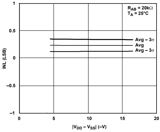
Figure 26. INL vs. Supply Voltage
