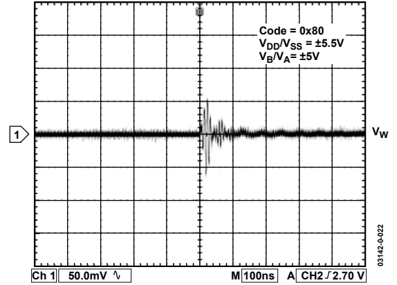
Figure 23. Digital Feedthrough
