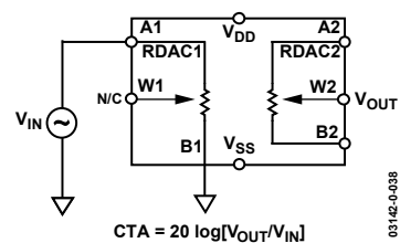
Figure 38. Test Circuit for Analog Crosstalk
