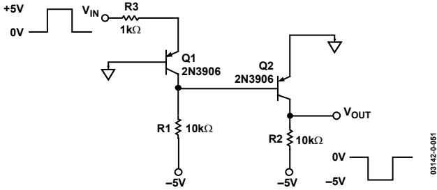
Figure 50. Level Shift for Bipolar Potential Operation
