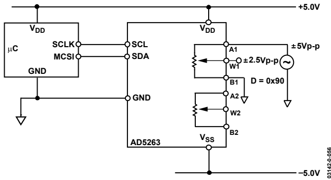
Figure 56. Bipolar Operation from Dual Supplies
