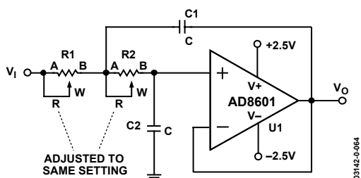
Figure 64. Sallen-Key Low-Pass Filter
