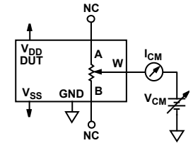
Figure 36. Test Circuit for Common Mode Leakage Current
