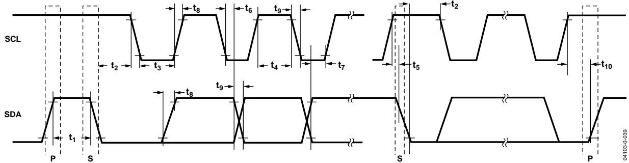
Figure 51. I 2 C Interface Detailed Timing Diagram
