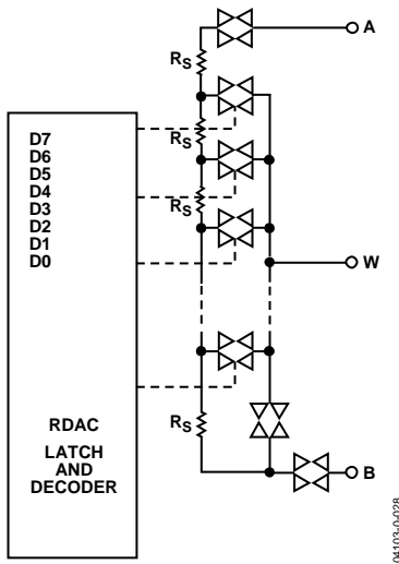
Figure 39. AD5172/AD5173 Equivalent RDAC Circuit
