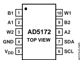
Figure 3. AD5172 Pin Configuration
