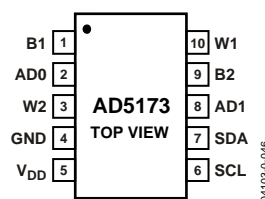
Figure 4. AD5173 Pin Configuration
