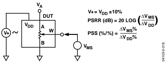
Figure 32. Power Supply Sensitivity (PSS, PSRR)
