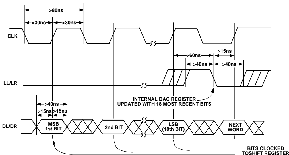
Figure 10. Timing Diagram
