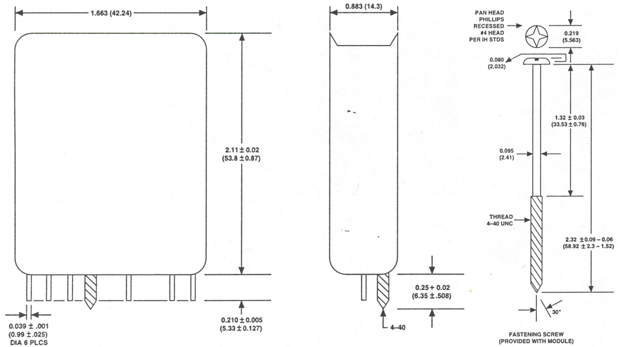
Figure 5. Outline Dimensions
