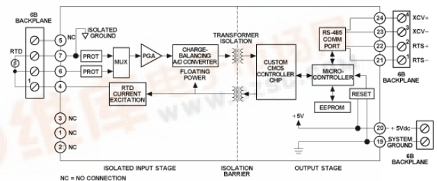
Figure 1. 6B13 & 6B13HV Functional Block Diagram
