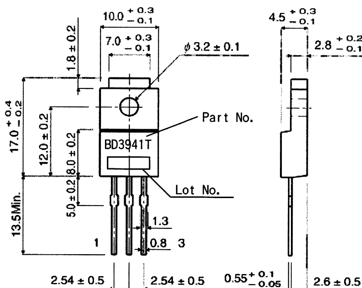
T0220FP (Unit:mm)
