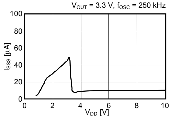
(2) Current Consumption at Shutdown ( I_{SSS} ) vs. Power Supply Voltage ( V_{DD} )
