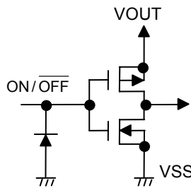
Figure 10 ON/OFF Pin Structure
