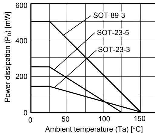
Figure 7 Power Dissipation of The Packages (Before Mounting)
