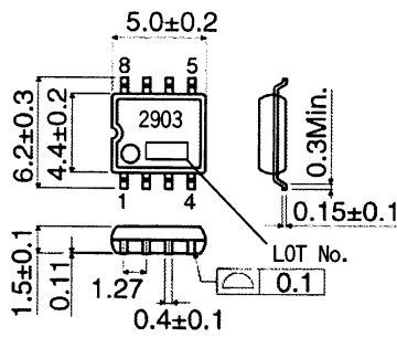
BA2903F(SOP8) (Unit:[mm])
