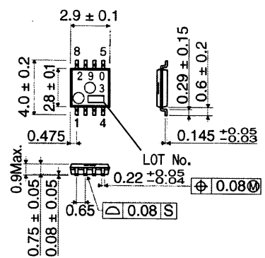
BA2903FVM(MSOP8)-(Unit:[mm])
