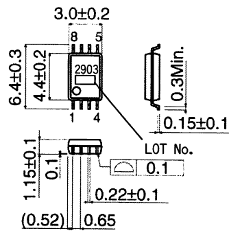
BA2903FV(SSOP-B8) (Unit:[mm])
