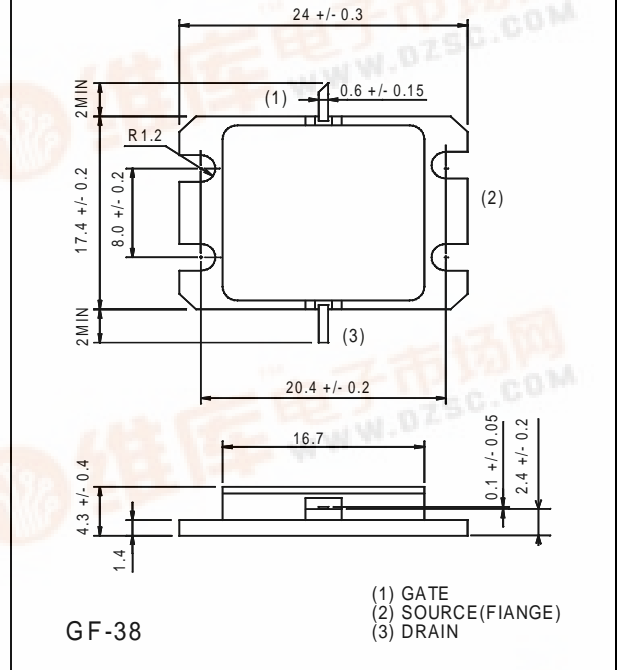
OUTLINE DRAWING Unit:millimeters (inches)
