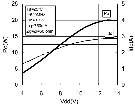
Vdd-Po CHARACTERISTICS @f=520MHz
