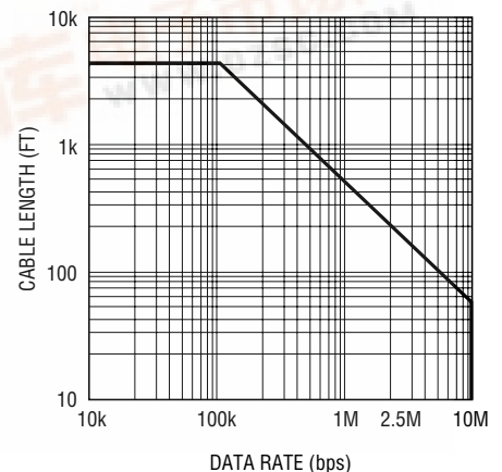
RS485 Cable Length Specification*
