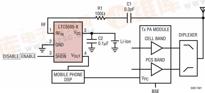
Dual Band Mobile Phone Tx Power Control
