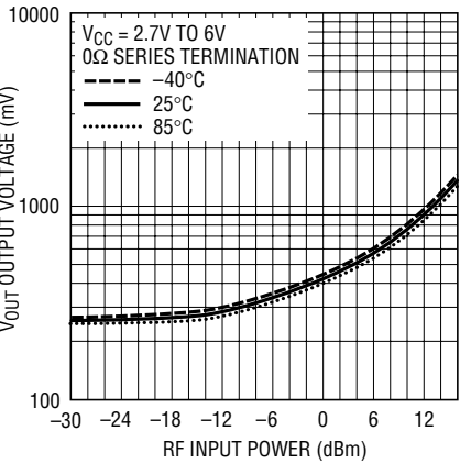
LTC5505-1 Typical Detector Characteristics, 2.45GHz
