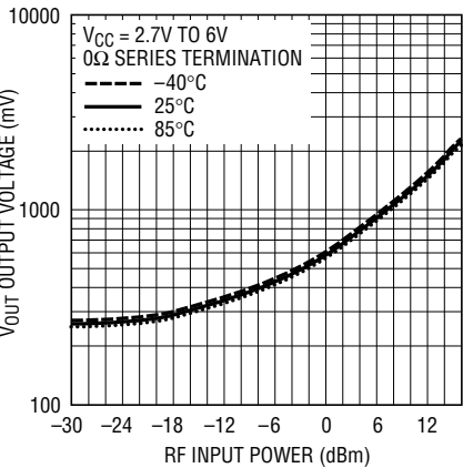
LTC5505-1 Typical Detector Characteristics, 0.85GHz
