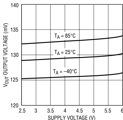
Output Starting Voltage vs Supply Voltage (RF Input Signal Off, V_{\text{OS}} = 0\text{V} )
