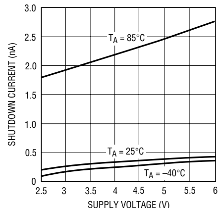
Shutdown Current vs Supply Voltage (RF Input Signal Off, V_{\text{OS}} = 0\text{V} , \overline{\text{SHDN}} = 0\text{V} )
