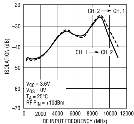
Channel-to-Channel Isolation vs RF Input Frequency
