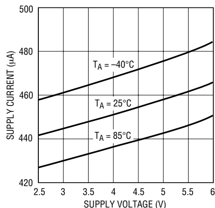
Supply Current vs Supply Voltage (RF Input Signal Off, V_{\text{OS}} = 0\text{V} )
