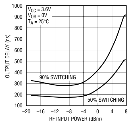
Output Delay vs RF Input Power
