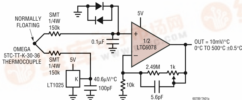
Thermocouple Signal Conditioner
