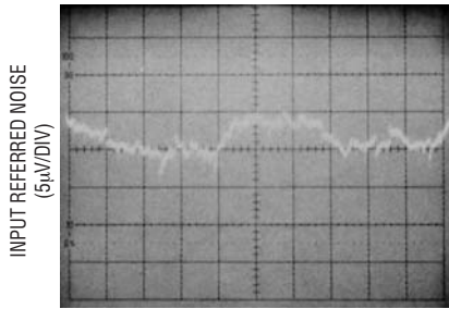
Broadband Noise, C_{EXT} = 0.1\mu F
