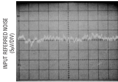
Broadband Noise, C_{EXT} = 1.0\mu F
