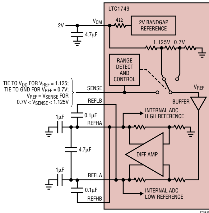
Figure 5. Equivalent Reference Circuit
