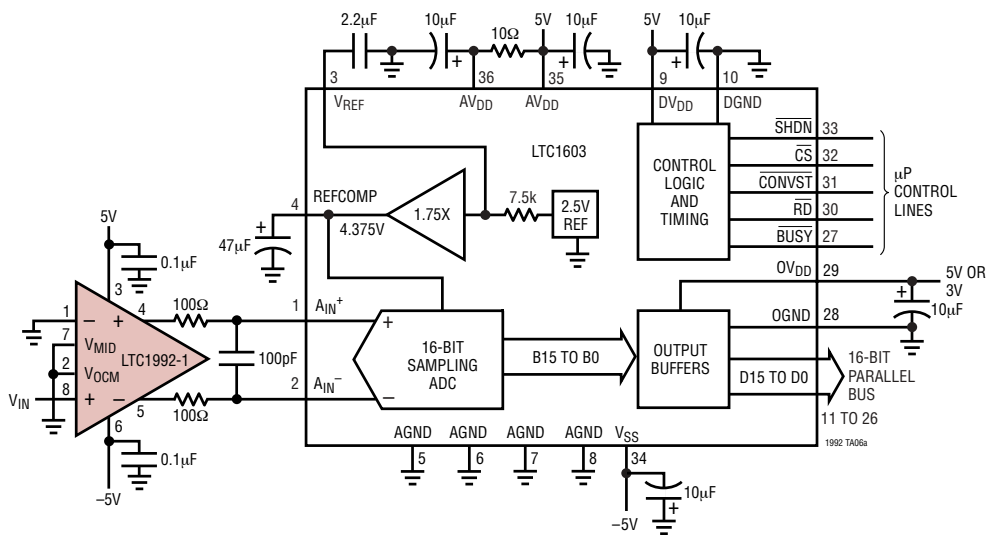
Single-Ended to Differential Conversion Driving an ADC
