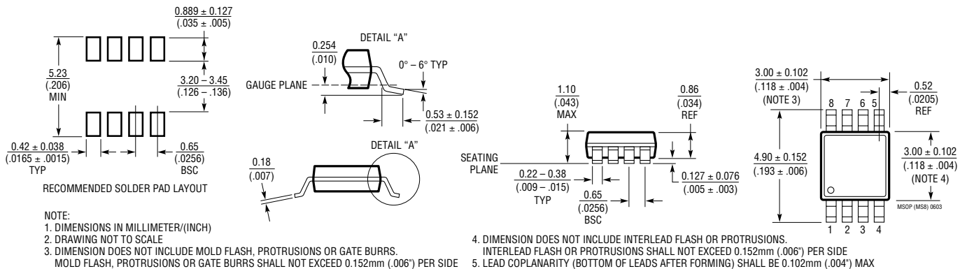
MS8 Package 8-Lead Plastic MSOP (Reference LTC DWG # 05-08-1660)
