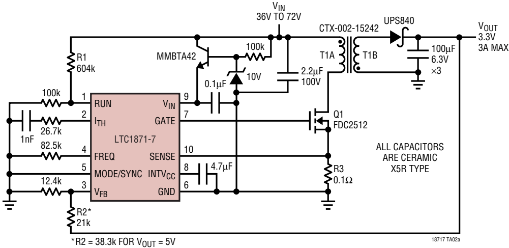
A 48V Input Flyback Converter Configurable to 3.3V or 5V Outputs
