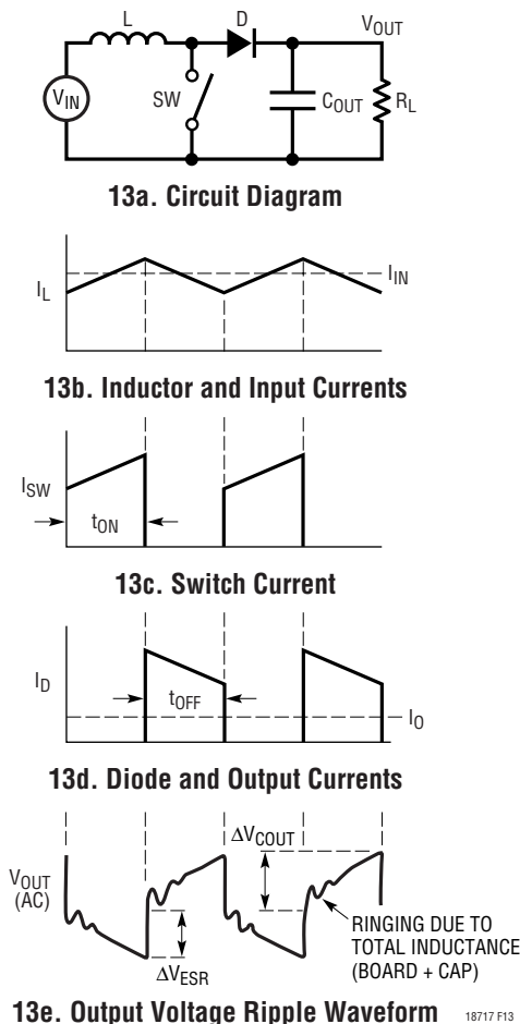
Figure 13. Switching Waveforms for a Boost Converter
