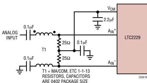
Figure 7. Recommended Front End Circuit for Input Frequencies Between 170MHz and 300MHz
