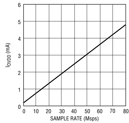
LTC2228: I_{VDD} vs Sample Rate, 5MHz Sine Wave Input, -1dB, O_{VDD} = 1.8\text{V}
