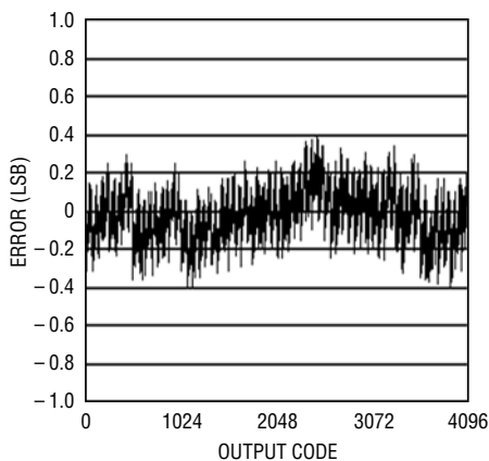
LTC2220: INL, 2V Range
