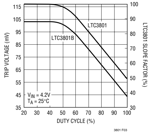
Figure 3. Maximum Current Limit Trip Voltage vs Duty Cycle
