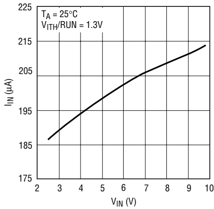
Input DC Supply Current (Normal) vs Input Voltage
