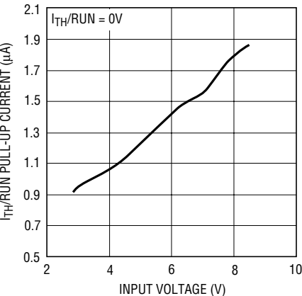
ITH/RUN Start-Up Current vs Input Voltage
