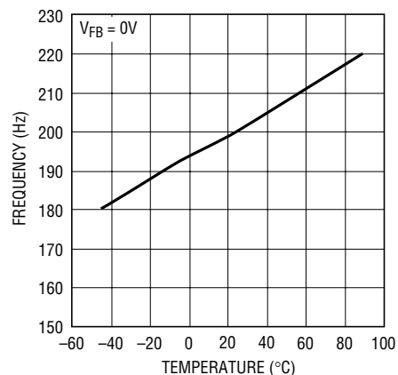
Foldback Frequency vs Temperature
