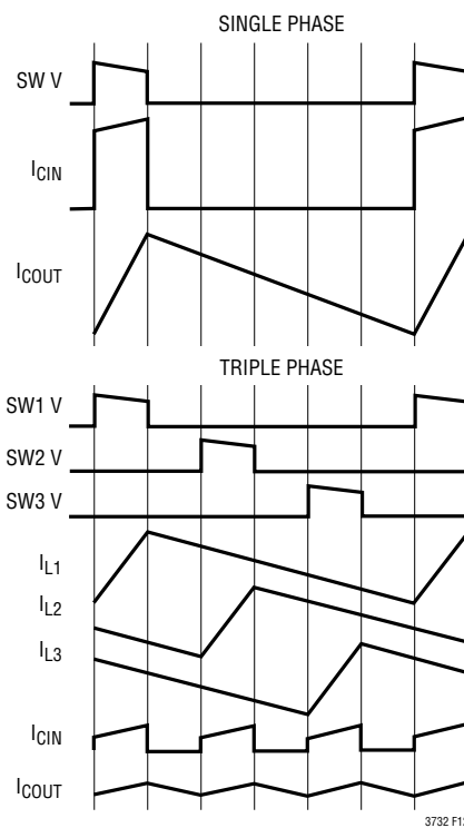
Figure 12. Single and Polyphase Current Waveforms
