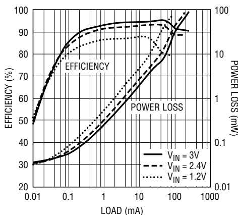
LTC3525-3.3 Efficiency and Power Loss vs Load
