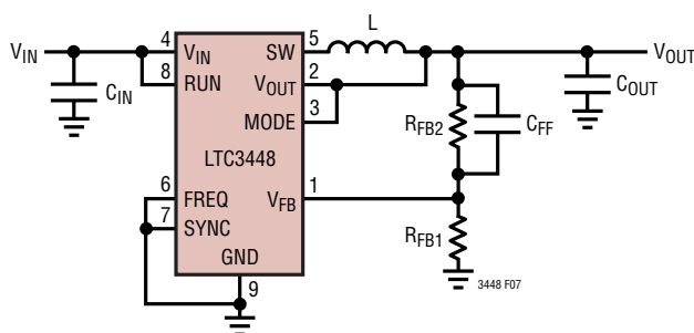
Figure 7. LTC3448 Layout Design
