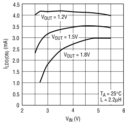
Figure 2. I_{LDO(ON)} vs V_{IN} , V_{OUT}
