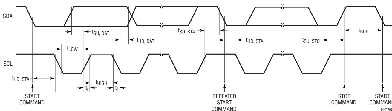
Figure 1. Timing Diagram
