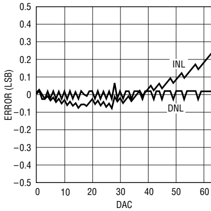
DAC Nonlinearity
