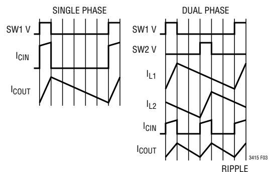
Figure 3. Single and 2-Phase Current Waveforms
