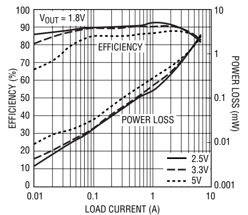
Efficiency and Power Loss Burst Mode Operation
