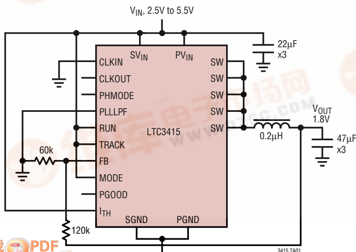
Figure 1. High Efficiency Step-Down Converter
