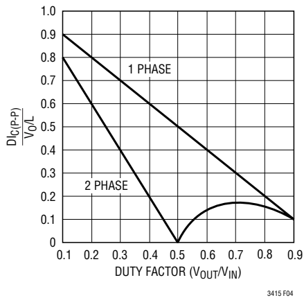
Figure 4. Normalized Output Ripple Current vs Duty Factor [ I_{RMS} \approx 0.3 (Dl_C(PP)) ]
