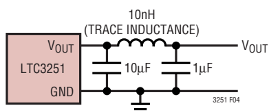
Figure 4. 10nH Inductor Used for Additional Output Noise Reduction
