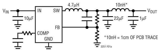
Figure 1a. Conventional Buck Switching Converter
