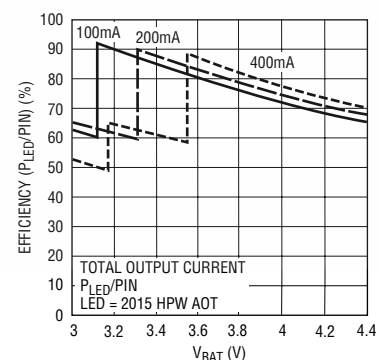
Efficiency vs V_{BAT}
