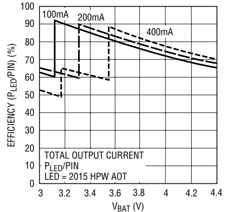
Efficiency vs V BAT
