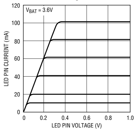
LED Pin Current vs LED Pin Voltage
