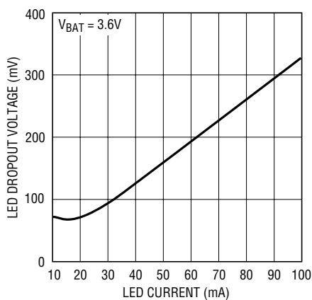
LED Dropout Voltage vs LED Current
