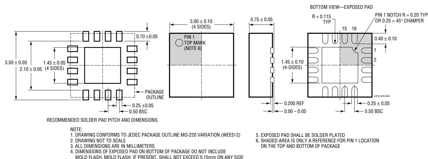
UD Package 16-Lead Plastic QFN (3mm × 3mm) (Reference LTC DWG # 05-08-1691)
