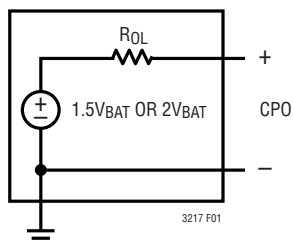
Figure 1. Equivalent Open-Loop Circuit
