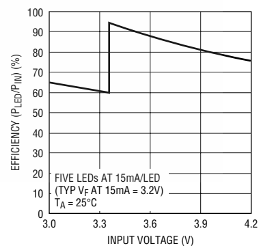
5-LED Main Display Efficiency vs Input Voltage
