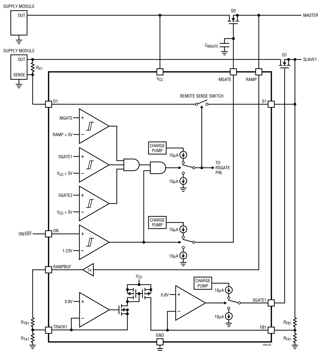
Figure 6. Simplified Functional Block Diagram
