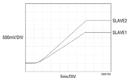
Figure 2. Ratiometric Tracking
