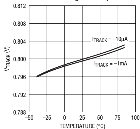
Track Pin Voltage vs Temperature
