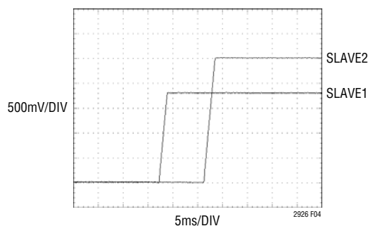
Figure 4. Supply Sequencing
