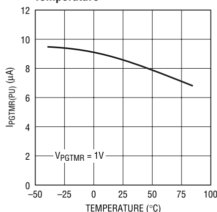
PGTMR Pin Pull-Up Current vs Temperature
