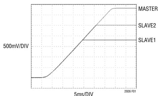
Figure 1. Coincident Tracking
