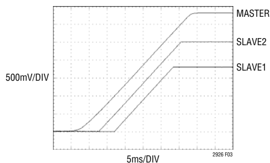
Figure 3. Offset Tracking
