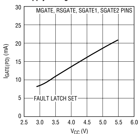
Gate Fault Pull-Down Currents vs Supply Voltage
