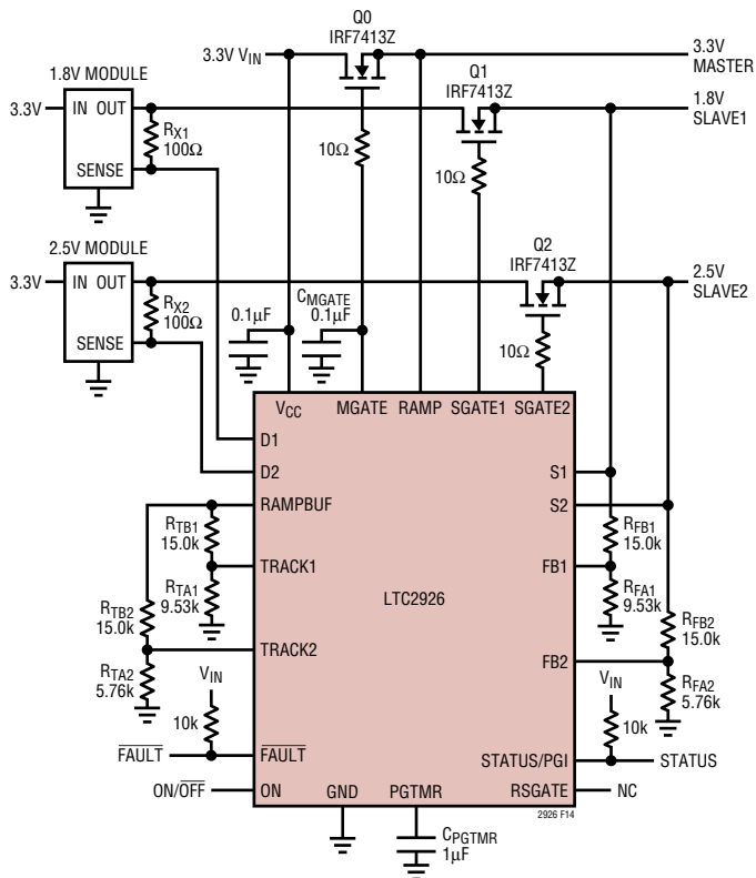
Figure 14. Coincident Tracking Example
