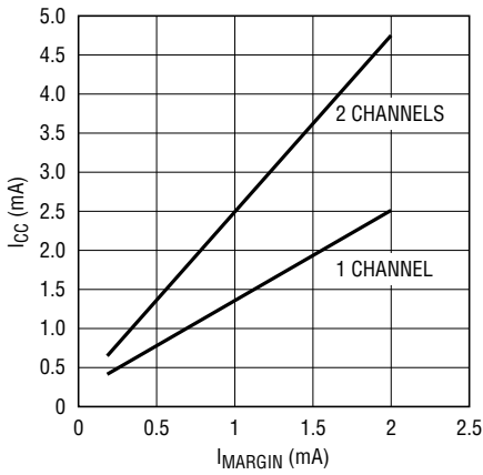
I_{CC} vs I_{MARGIN} High Range Sourcing Current
