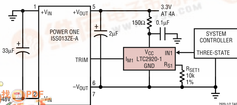
3.3V Quarter Brick with ±5% Voltage Margining
