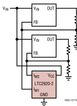
Figure 16. Connecting V_{CC} to V_{IN}
