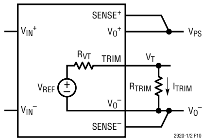
Figure 10. Power Module I_{\text{TRIM}} Model
