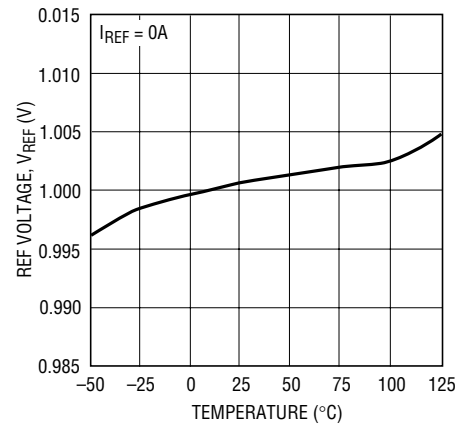
REF Output Voltage vs Temperature
