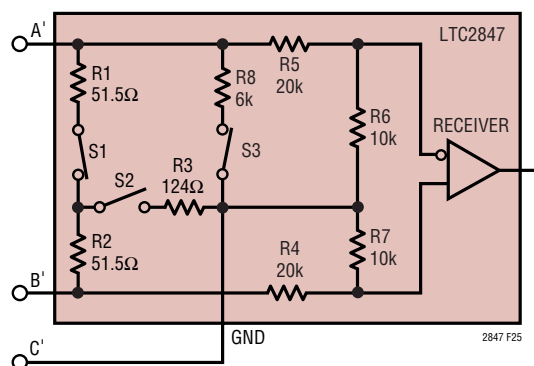
Figure 25. V.28 Receiver Configuration
