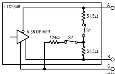
Figure 20. V.35 Driver
