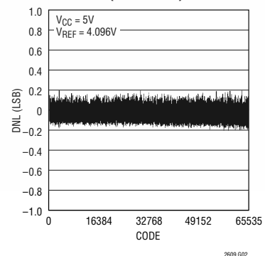
Differential Nonlinearity (LTC2609)
