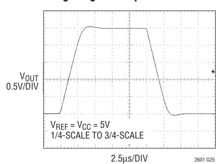
Large-Signal Response
