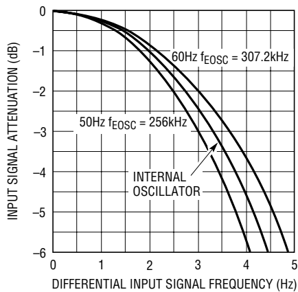
Figure 24. Input Signal Using the Internal Oscillator
