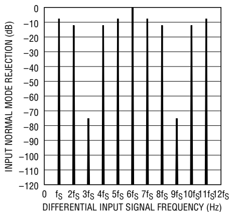
Figure 26. Input Normal Mode Rejection, External Oscillator ( f_{EOSC} = 256\text{kHz} ) 50Hz Rejection
