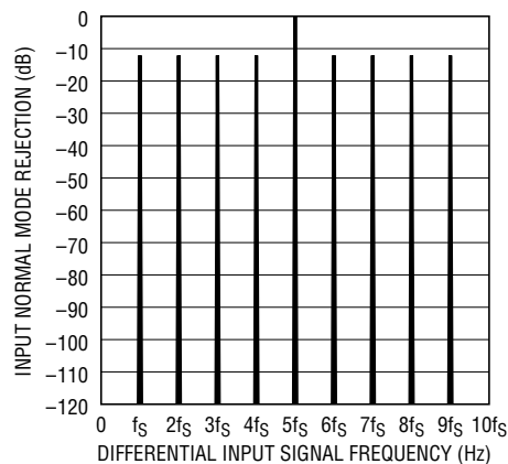
Figure 27. Input Normal Mode Rejection at DC (Internal Oscillator)
