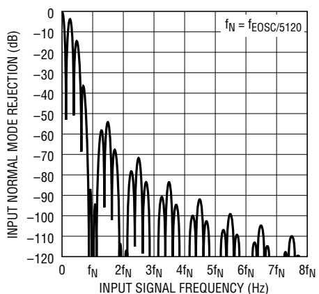
Figure 28. Input Normal Mode Rejection at DC
