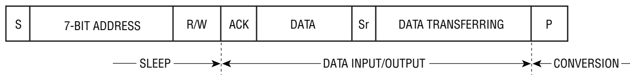
Figure 4. The LTC2483 Conversion Sequence
