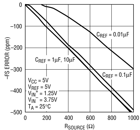
Figure 19. -FS Error vs R SOURCE at REF + or REF - (Large C REF )
