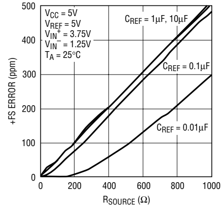
Figure 18. +FS Error vs R SOURCE at REF + or REF - (Large C REF )
