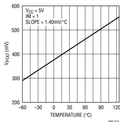
Figure 11. Internal PTAT Signal vs Temperature
