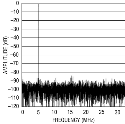
LTC2288: 8192 Point FFT, f_{IN} = 70\text{MHz} , -1dB, 2V Range, 65Mps
