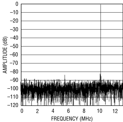
LTC2286: 8192 Point FFT, f_{IN} = 140\text{MHz} , -1\text{dB} , 2\text{V} Range, 25\text{Mpsps}
