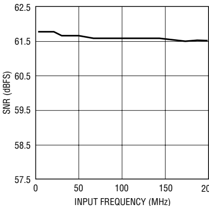
LTC2286: SNR vs Input Frequency, -1\text{dB} , 2\text{V} Range, 25\text{Mpsps}
