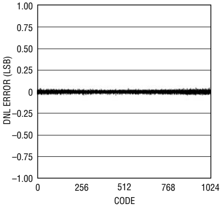
LTC2288: Typical DNL, 2V Range, 65Mps
