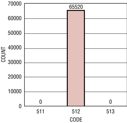
LTC2288: Grounded Input Histogram, 65Mps
