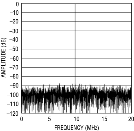
LTC2287: 8192 Point FFT, f_{IN} = 70\text{MHz} , -1dB, 2V Range, 40Msps
