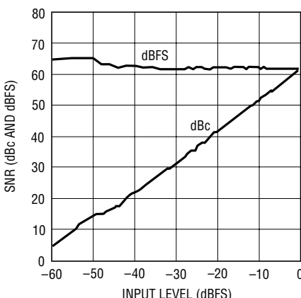
LTC2286: SNR vs Input Level, f_{IN} = 5\text{MHz} , 2\text{V} Range, 25\text{Mpsps}
