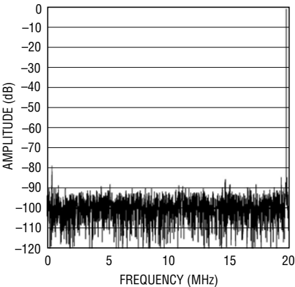
LTC2287: 8192 Point FFT, f_{IN} = 140\text{MHz} , -1dB, 2V Range, 40Msps
