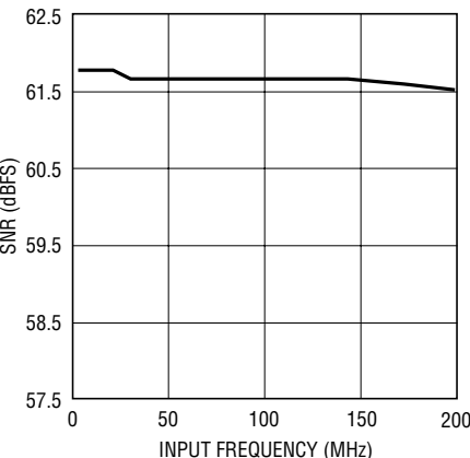
LTC2287: SNR vs Input Frequency, -1dB, 2V Range, 40Msps
