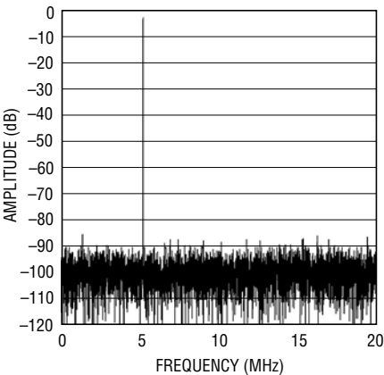
LTC2287: 8192 Point FFT, f_{IN} = 5\text{MHz} , -1dB, 2V Range, 40Msps
