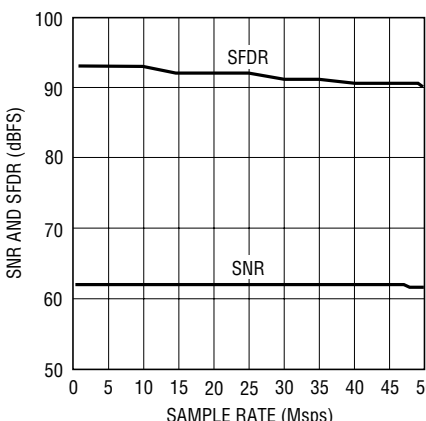
LTC2286: SNR and SFDR vs Sample Rate, 2\text{V} Range, f_{IN} = 5\text{MHz} , -1\text{dB}
