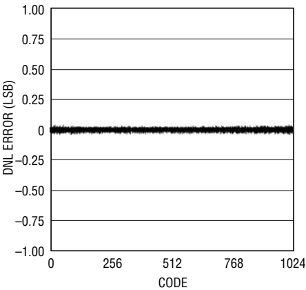
LTC2287: Typical DNL, 2V Range, 40Msps
