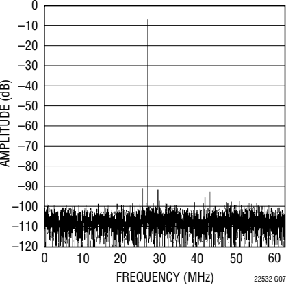
LTC2253: 8192 Point 2-Tone FFT, f_{IN} = 28.2\text{MHz} and 26.8\text{MHz} , -1dB, 2V Range, 125Mps
