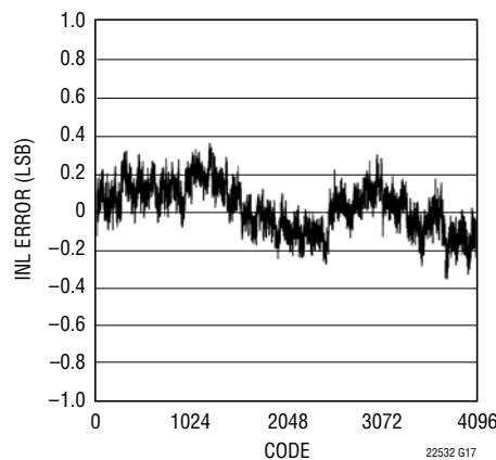
LTC2252: Typical INL, 2V Range, 105Msps
