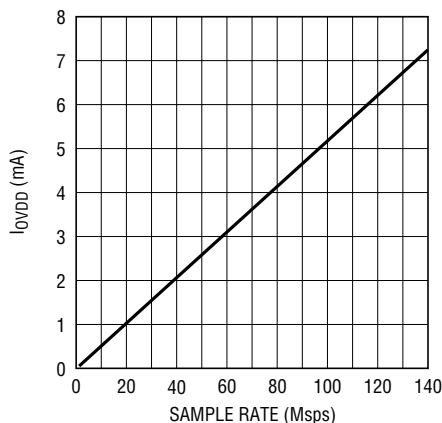
LTC2253: I_{OVD} vs Sample Rate, 5MHz Sine Wave Input, -1dB, O_{VDD} = 1.8\text{V}
