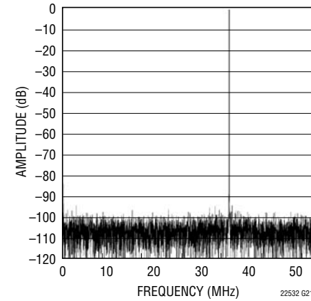
LTC2252: 8192 Point FFT, f_{IN} = 70\text{MHz} , -1dB, 2V Range, 105Msps
