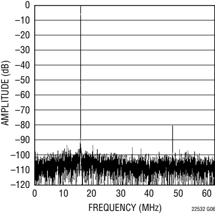
LTC2253: 8192 Point FFT, f_{IN} = 140\text{MHz} , -1dB, 2V Range, 125Mps
