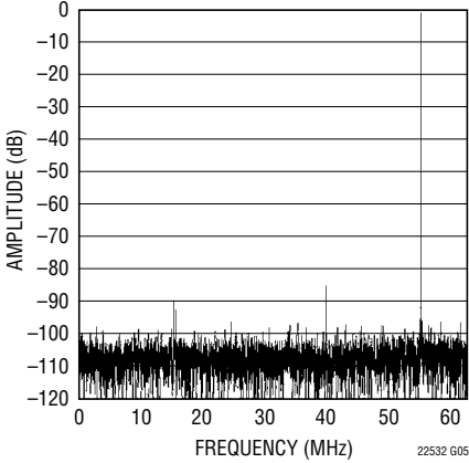
LTC2253: 8192 Point FFT, f_{IN} = 70\text{MHz} , -1dB, 2V Range, 125Mps
