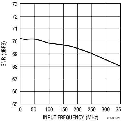
LTC2252: SNR vs Input Frequency, -1dB, 2V Range, 105Msps
