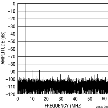
LTC2253: 8192 Point FFT, f_{IN} = 5\text{MHz} , -1dB, 2V Range, 125Mps
