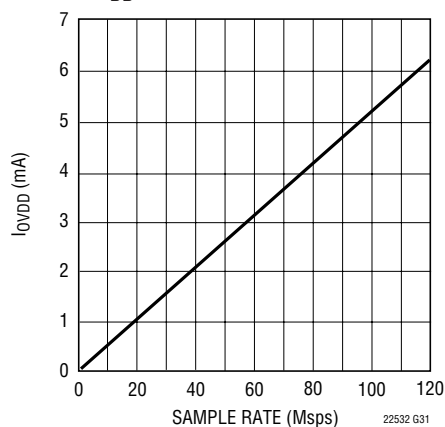
LTC2252: I_{OVD0} vs Sample Rate, 5MHz Sine Wave Input, -1dB, OV_{DD} = 1.8\text{V}
