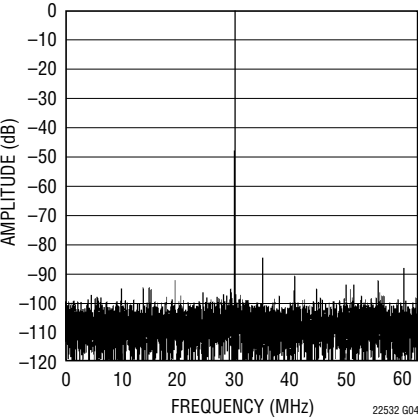
LTC2253: 8192 Point FFT, f_{IN} = 30\text{MHz} , -1dB, 2V Range, 125Mps
