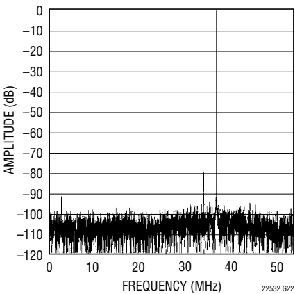
LTC2252: 8192 Point FFT, f_{IN} = 140\text{MHz} , -1dB, 2V Range, 105Msps
