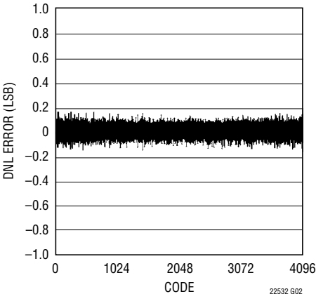
LTC2253: Typical DNL, 2V Range, 125Mps
