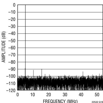
LTC2252: 8192 Point FFT, f_{IN} = 5\text{MHz} , -1dB, 2V Range, 105Msps
